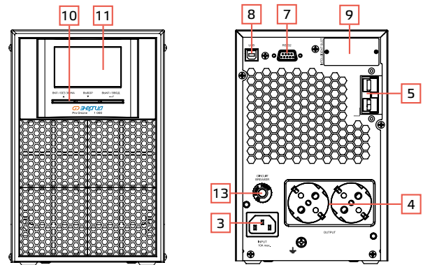
Pro Online 1000 230 B – 24 B Tower
